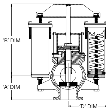
DOUBLE SPRING STACK (HIGHER PRESSURE RANGES)
