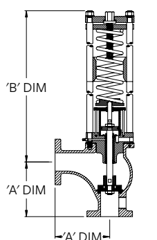
SINGLE SPRING STACK (LOWER PRESSURE RANGES)
